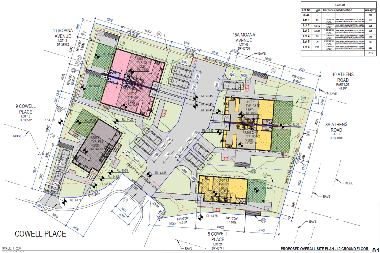
Figure 1: Site Plan
